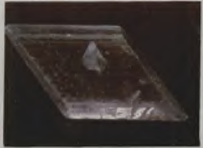
Gips.
